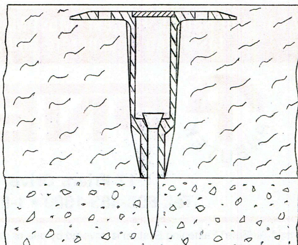
XIW INSTALLED IN CONCRETE
