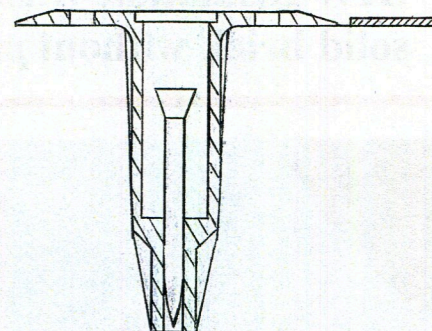
XIW WASHER/FASTENER ASS'Y
